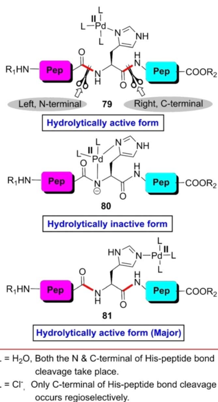
Fig. 6 Modes of co-ordination of Pd(II)-complex with histidiny peptide. Reaction conditions: (a) histidiny peptide, cis\text{-[Pd(en)(H}_2\text{O)}_2\text{]}^{2+} , \text{HBF}_4 (promoter), pH 1.5–2 (0.1 M HCl or 70% \text{HCOOH} ), 40 °C, 2 days, 60–80%.
