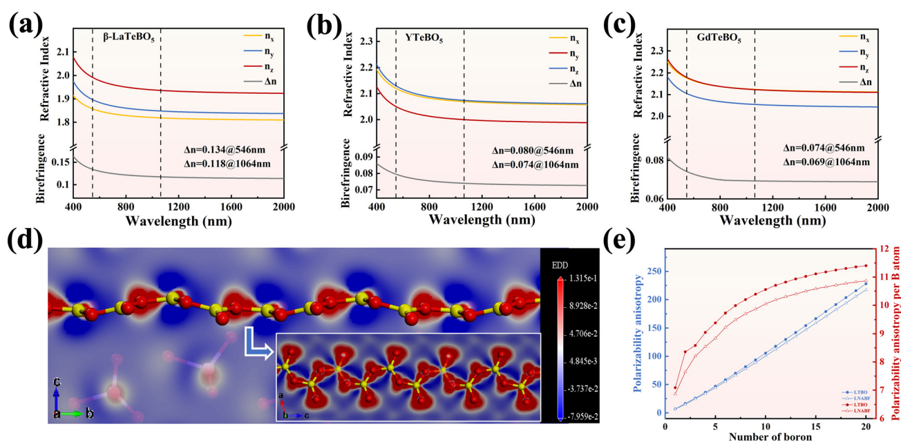
Fig. 7 Calculated refractive indices and birefringence values for \beta -LaTeBO 5 (a), YTeBO 5 (b), and GdTeBO 5 (c). Electron density difference maps of the ^1[\text{BO}_2]_\infty chain in \beta -LaTeBO 5 (d). Polarizability anisotropy and permutation contribution rate in \beta -LaTeBO 5 and \text{Li}_{0.5}\text{Na}_{0.5}\text{AlB}_2\text{O}_4\text{F}_2 depending on the numbers of boron atoms in \text{B}_n\text{O}_{2n+1} ( n = 1, 2, \dots, 20 ) (e).
