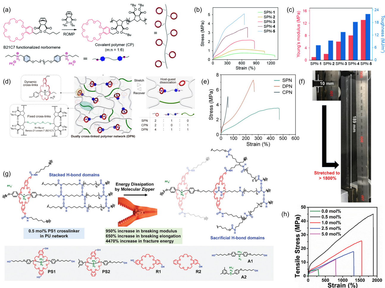
Fig. 32 (a) Synthesis of supramolecular networks (SPNs) composed of B21C7-norbornene-based hosts and dialkylammonium guests. (b) Uniaxial tensile tests of SPN- x (molar ratio of guest: host = x :10) shows increasing toughness and yield strength with increasing guest concentration. (c) Comparative studies show increasing Young's modulus and tensile toughness with an increasing concentration of host-guest interactions. Figure adapted from ref. 162. (d) Dually cross-linked polymers with both supramolecular and covalent cross-links. Three polymers (SPN, CPN and DPN) were constructed with different compositions of supramolecular and covalent networks. (e) Tensile tests comparing the mechanical performance of SPN, CPN and DPN show DPN having higher overall toughness. Figure adapted from ref. 163. Copyright 2023 Wiley-VCH GmbH. (f) PPS1 can be extended to a length of more than 1800% without fracturing. (g) Scheme showing the design of zipper gels with monomers PS1 and PS2 as well as controls R1, R2, A1 and A2. (h) Mechanical performance of PPS1 gels with different concentrations of PS1. Figure adapted from ref. 164. Copyright 2020 WILEY-VCH Verlag GmbH & Co. KGaA, Weinheim.
