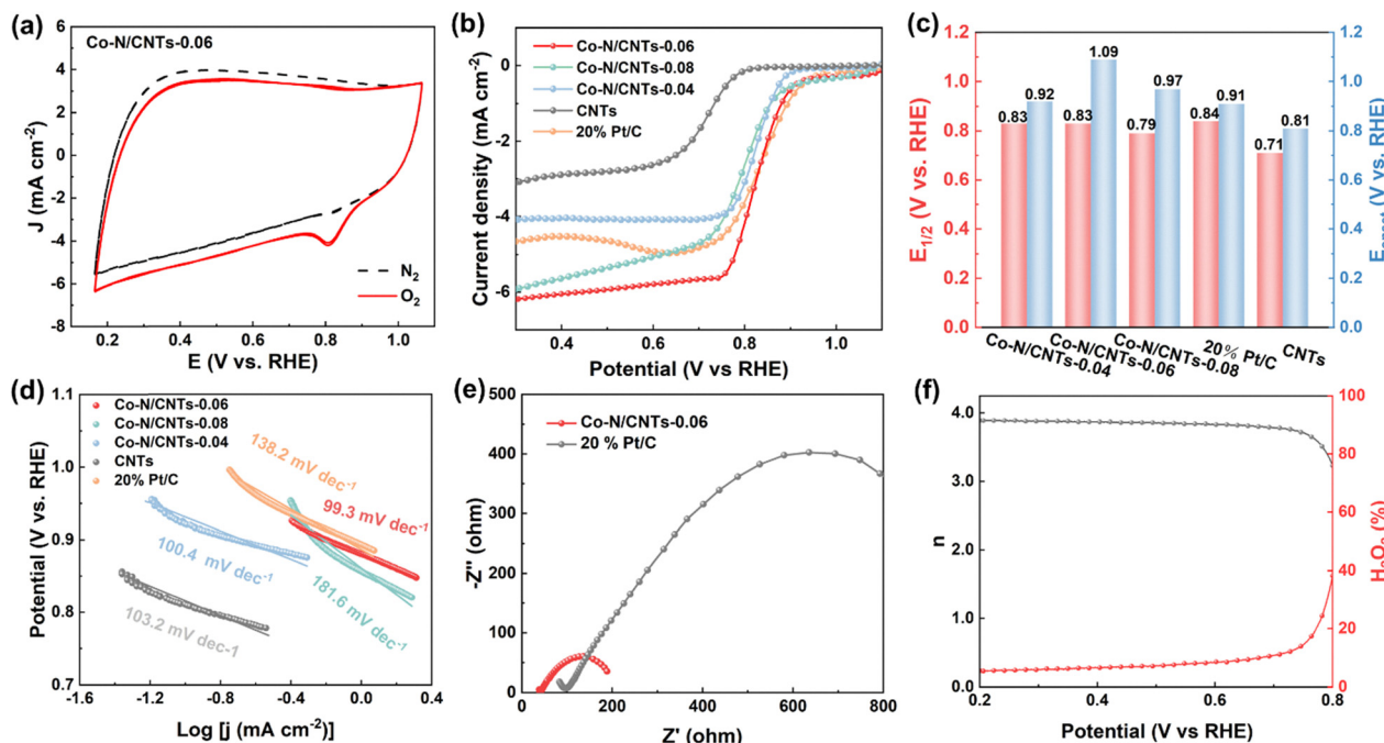
Fig. 3 (a) CV curves of Co-N/CNTs-0.06 in N 2 - and O 2 -saturated 0.1 M KOH at the scan rate of 10 mV s -1 . (b) The linear sweep voltammetry (LSV) curves, (c) the half-wave potential and onset potential, and (d) Tafel plots of the ORR on CNTs, Co-N/CNTs-0.04, Co-N/CNTs-0.06, Co-N/CNTs-0.08, and 20% Pt/C in 0.1 M KOH solution at 1600 rpm. (e) EIS pattern of Co-N/CNTs-0.06 and 20% Pt/C recorded at 1.03 V vs. RHE. (f) Calculated n and determined H 2 O 2 % at various potentials based on the RRDE.
