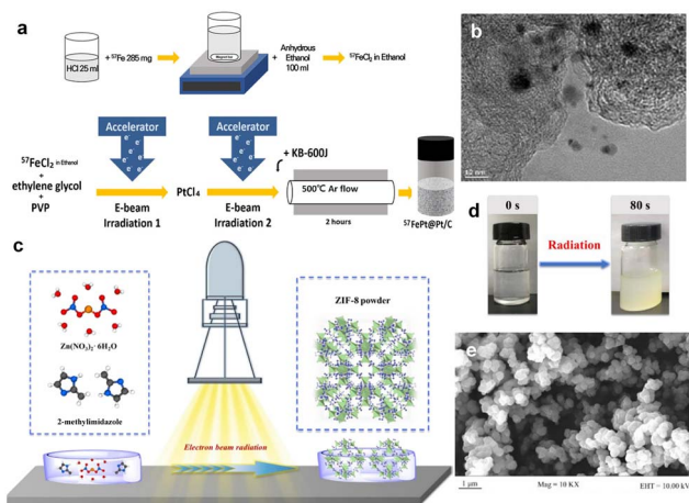
Fig. 4 (a) Schematic illustration of the synthesis of 57FePt@Pt/C via electron-beam irradiation. (b) TEM image of 57FePt@Pt/C. Copyright 2023 Wiley-VCH. (c) The synthesis setup of ZIF-8 via electron beam radiation. (d) The photo of ZIF-8 synthesized at an absorbed dose of 50 kGy. (e) SEM image of ZIF-8 at an absorbed dose of 50 kGy. 54,55 Copyright 2022, Wiley-VCH.
