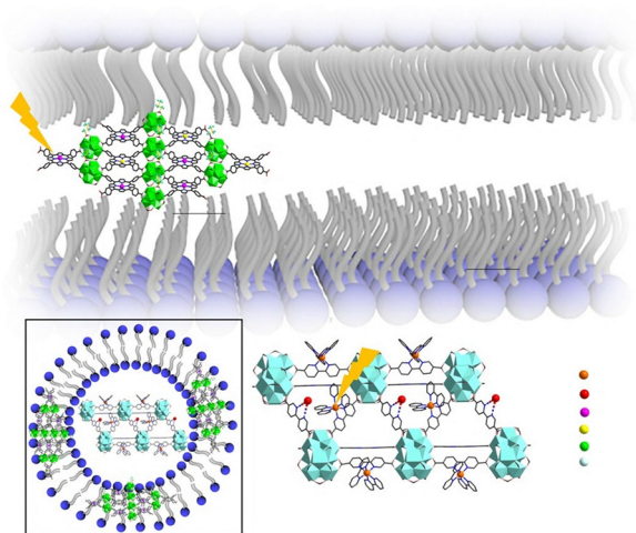
Fig. 21 Structure of the LP-MOF for overall photocatalytic water splitting and the proposed 'Z-scheme' electron-transfer chain in the LP-MOF system. The bilayer in the illustration represents a section of the liposome. The HER-MOF for hydrogen evolution is incorporated between the hydrophobic chains, and the WOR-MOF for water oxidation is in the aqueous phase. The redox shuttles TCBQ/TCBQH and \text{Fe}^{3+}/\text{Fe}^{2+} connect the HER and WOR sides, functioning in the lipid phase and the aqueous phase, respectively. Electron-transfer chains (shown by blue arrows) and photons (represented by yellow lightning shapes) form the 'Z-scheme'. Inset, schematic representation of the liposome with the two MOFs embedded within the hydrophobic bilayer (HER-MOF) and the hydrophilic interior (WOR-MOF). 187 Copyright 2021, Nature.
