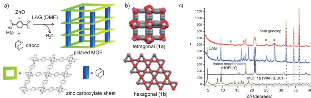
Fig. 7 (a) Expected MOF 1 assembly; (b) MOF isomers 1a and 1b; red O, gray C, blue N, purple Zn. (c) PXRD patterns (top to bottom): 60 min neat grinding (red; no reaction), 60 min LAG (blue; partial reaction), simulated pattern for the dabco-Hta salt and for 1b (in square-root scale). Dotted lines indicate reflections of ZnO; reflections of residual Hta are labeled "☆". 147 Copyright 2010, Wiley.
