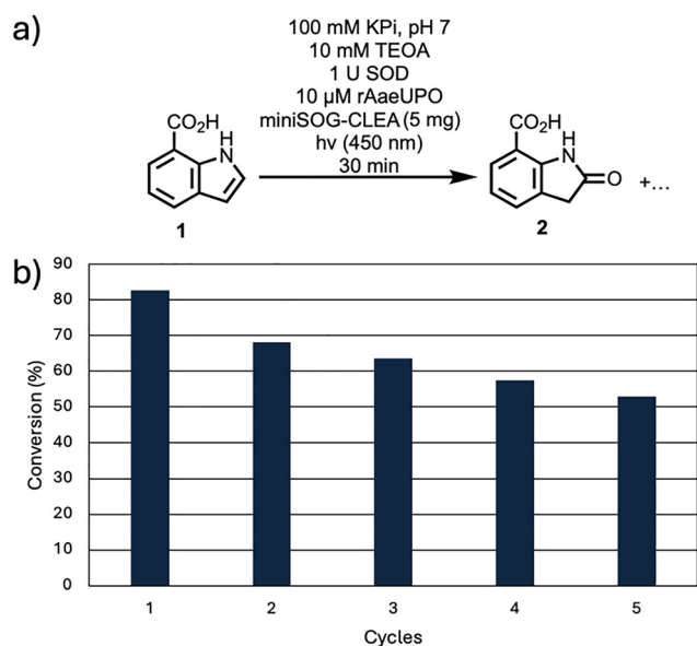
Fig. 4 (a) Reaction scheme and conditions for the blue-light mediated oxidation of 1 (1 mM) to oxindole 2 using rAaeUPO and in situ produced H 2 O 2 from miniSOG-CLEA. (b) Recyclability test of the miniSOG-CLEA photocatalyst.
