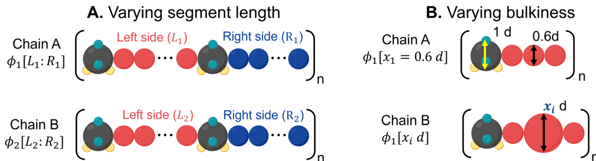
Fig. 7 (A) Mixtures of varying segment lengths. Chain A consists of a monomer with [L_1, R_1] , i.e., L_1 CH 2 beads on the left side and R_1 CH 2 beads on the right side of the sulfamide, respectively, while Chain B consists of a monomer with [L_2, R_2] , i.e., L_2 CH 2 beads on the left side and R_2 CH 2 beads on the right side of the sulfamide, respectively. The total number of CH 2 beads in the monomer is kept constant. \phi_1 and \phi_2 represent the volume percent of Chain A and Chain B in the polymer mixture. (B) Mixtures of varying bulkiness in the backbone. Chain A has a fixed bead size, where all beads are 0.6d , while in Chain B, the size of the center bead is varied ( x_1 ). \phi_1 and \phi_2 represent the volume percents of Chain A and Chain B in the polymer mixture.
