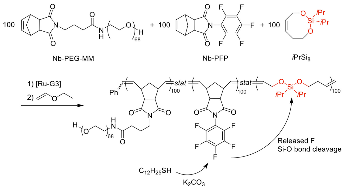
Fig. 23 Synthesis of a polynorbornene graft terpolymer containing PFP substituent, and its deconstruction by a S N Ar-triggered cascade. 59
