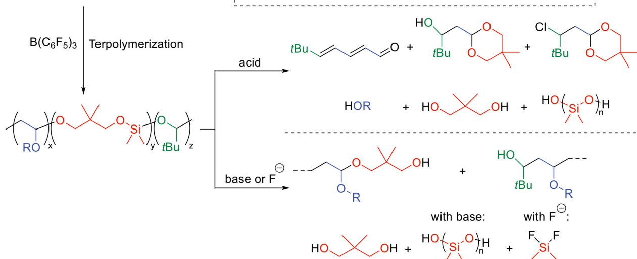
Fig. 17 Cationic polymerization of silyl ether-based poly(vinyl ether) and degradation of acetal and silyl ether groups in the backbone by acids, bases, or fluoride ions. 49
