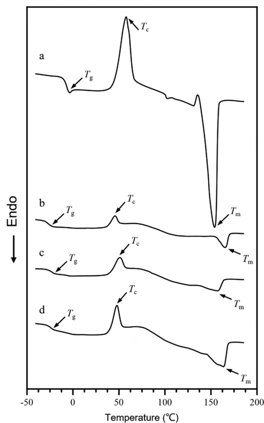
Fig. 8 Differential scanning calorimetry (DSC) thermographs of P3HB3H9Od containing different proportions of 3H9Od produced by H. bluephagenesis TXY32E. (a) P3HB. (b) P(3HB- co -5 mol% 3H9Od). (c) P(3HB- co -7.5 mol% 3H9Od). (d) P(3HB- co -10 mol% 3H9Od).
