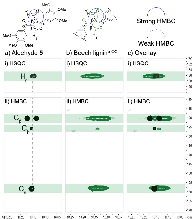
Figure 4. Identifying the furan-aldehyde unit in SiS lignin ox . Selected regions of the HSQC NMR ( ^1H/^{13}C / \delta 10.05 – 10.25 / 185 – 189 ppm, 700 MHz, d_6 -DMSO) analysis of: a) i) aldehyde 5 and b) i) beech lignin ox and c) i) an overlay of the two spectra indicating the presence of an aldehyde crosspeak in both. Selected regions of the HMBC NMR analysis ( ^1H/^{13}C / \delta 10.05 – 10.25/ 110 – 170 ppm, 700 MHz, d_6 -DMSO) of: A) ii) aldehyde 5 ; B) ii) beech lignin ox (generated using 3 wt. eq. of DDQ) and c) ii) an overlay of the two spectra indicating 3 key crosspeaks resulting from various strength couplings. For atom labelling see structures at top of figure.
