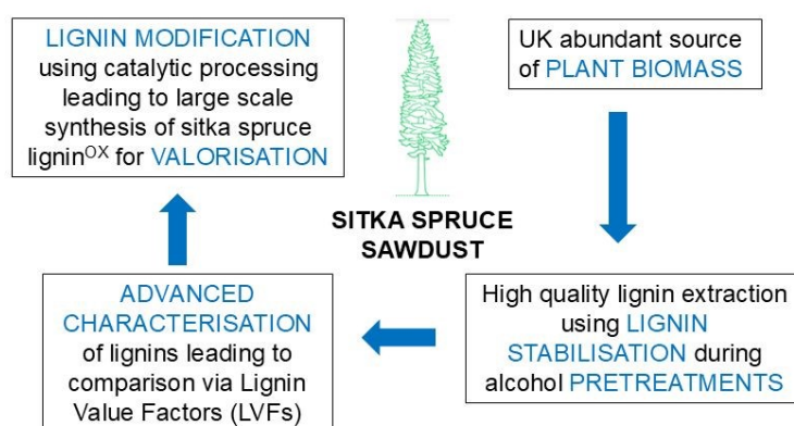
Figure 1. An overview of the research presented and its relevance to the various sections of the Frontiers in Physical Chemistry for Lignin Valorisation Faraday Discussion.
