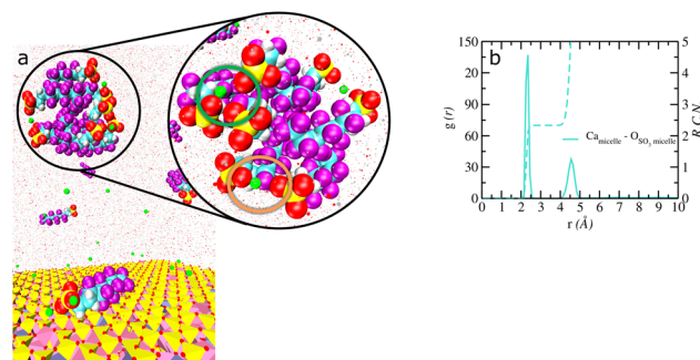
Fig. 7 Pictorial representations of the micellar type of structure of (a) 6:2 FTS in the solution phase of montmorillonite. b) Radial distribution functions (solid lines) and corresponding running coordination numbers (RCNs-dashed lines) between the solution cluster associated \text{Ca}^{2+} ions and the 'O' atoms of the 6:2 FTS belonging to the micellar type of structure in montmorillonite.
