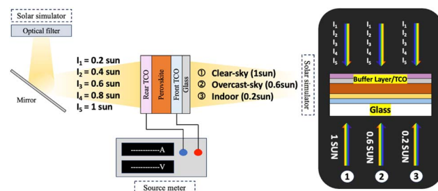
Fig. 11 Schematic measurement of bifacial illumination with simulated scenarios of clear sky, overcast sky, and indoor conditions.
