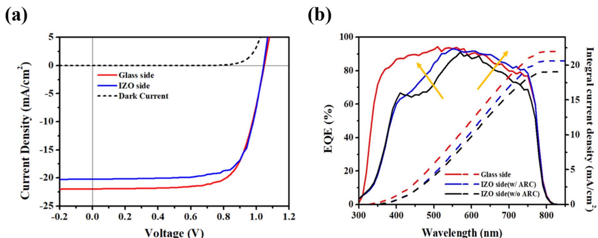
Fig. 9 (a) J - V curves and (b) EQE spectra of ALD SnO 2 bifacial device with an ARC illuminated with 1 sun from glass and IZO sides.
