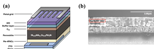
Fig. 1 Bifacial devices: (a) illustration and (b) cross-sectional SEM image.
