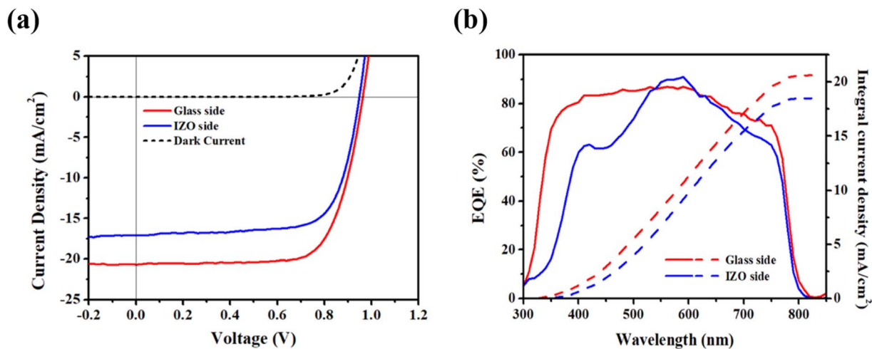
Fig. 8 (a) J - V curve and (b) EQE spectra of the ALD SnO 2 10 nm bifacial device under 1 sun illumination from glass and IZO sides.
