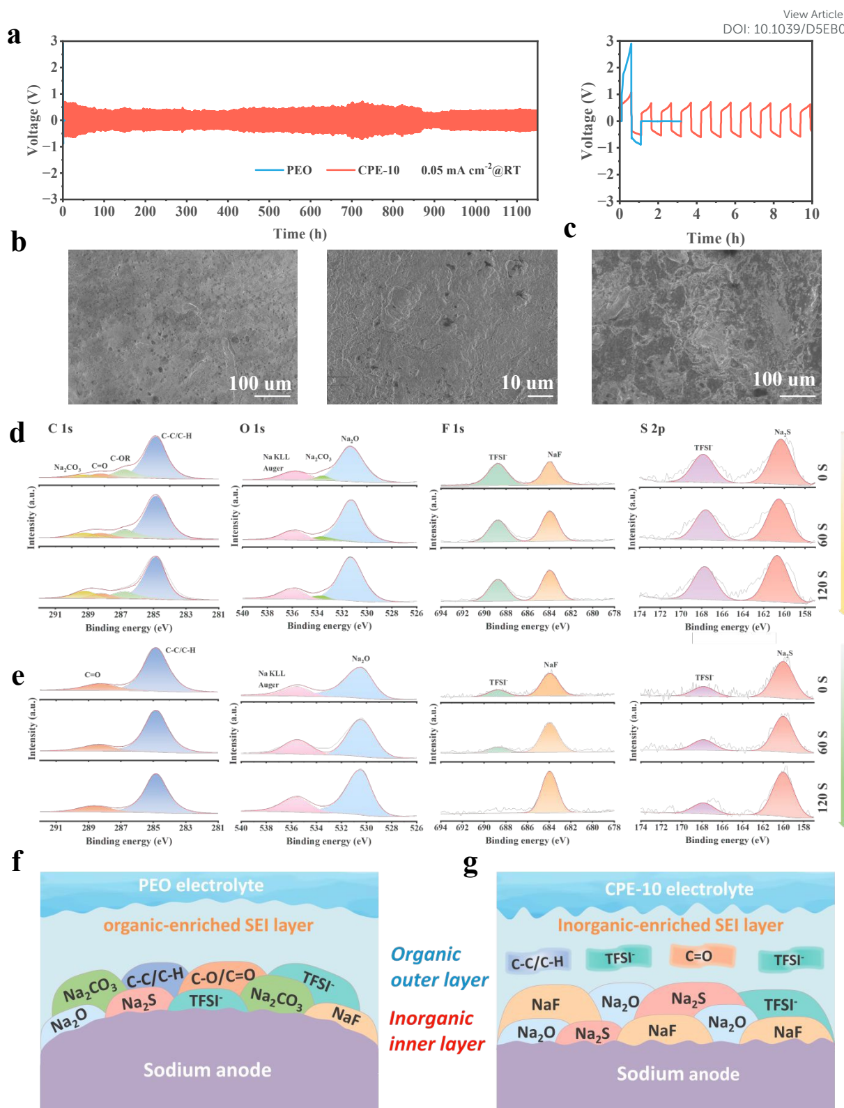
Figure 5. (a) Comparison of cycling performance of Na/Na symmetric cells with the CPE-10 and PEO electrolytes plating/stripping at 0.05 mA cm -2 for 30 min. The inset shows the enlarged view of cycle stages at 25 °C. The SEM images of Na anode after cycling for 50 h for (b) Na/CPE-10/Na and (c) Na/PEO/Na cells. Ex-situ XPS measurements of sodium metal anode surface, etched for 60 s and 120 s after cycling for 50 h for (d) PEO and (e) CPE-10 systems, with the signals of C 1s, O 1s, F 1s and S 2p. Schematic illustration of components at the surface of cycled sodium metal anode based on (f) PEO and (g) CPE-10.
