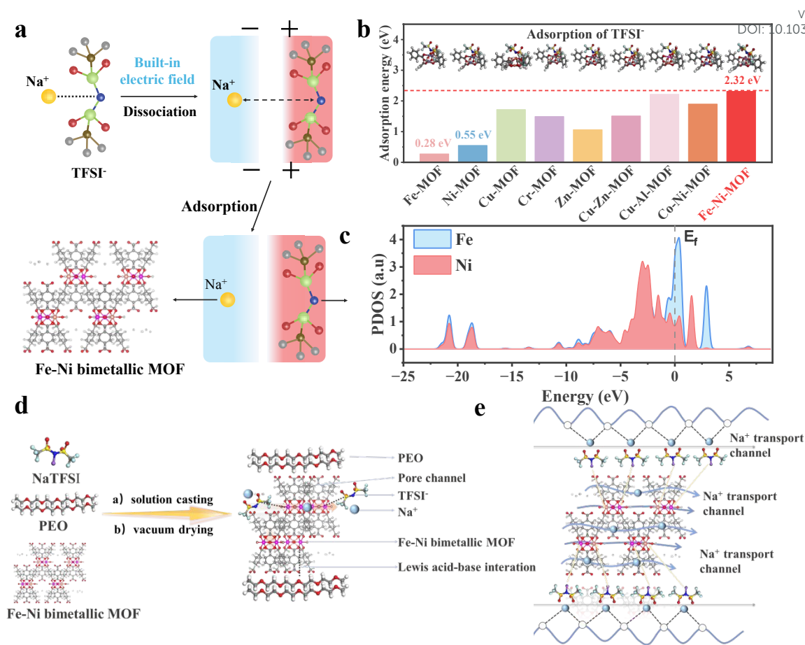
Figure 1. (a) Detailed depiction of the dissociation and adsorption mechanisms of NaTFSI. (b) Theoretical calculations that screen the adsorption energy of TFSI - on reported and representative single-metal and bimetallic MOFs. (c) DFT-calculated the DOS of MOF(Fe-Ni). (d) Schematic diagram of CPEs synthesis. (e) Schematic illustration of Fe-Ni MOF enhanced structure of CPEs with selective and rapid Na + transport.
