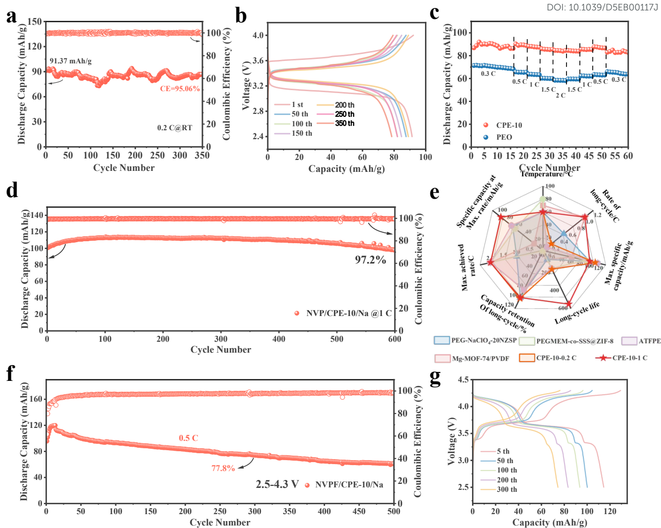
Figure 6. (a, b) Cycling performance of the NVP/CPE-10/Na cell at 25 °C with a current density of 0.2C. (c) Rate performances (0.3–2C) of the NVP/PEO/Na and NVP/CPE-10/Na cells. (d) Cycling performance of the NVP/CPE-10/Na cells at 60 °C and 1C. (e) Comparison of CPE-based cells with the previously reported ASSMBs in rate capability and long-term cycling performance. (f) Cycling performance of the NVPF/CPE-10/Na cells at 60 °C with a current density of 0.5C. (g) The corresponding voltage profile of the all-solid-state NVPF/CPE-10/Na at 0.5C in different cycles.
