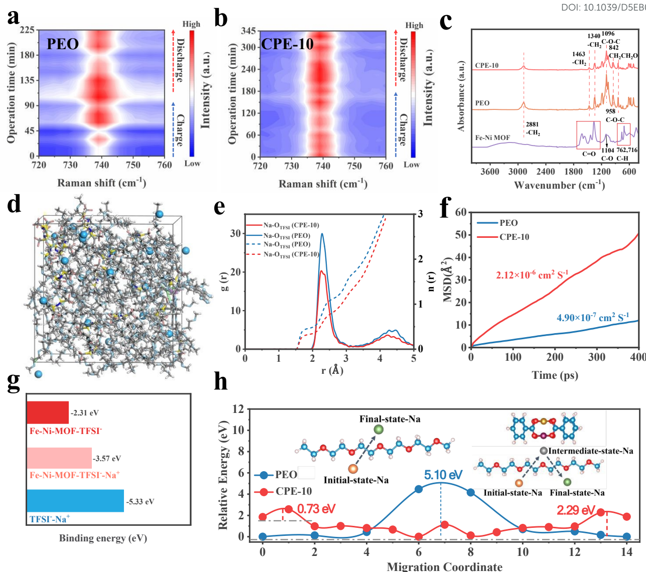
Figure 4. (a, b) In-situ Raman spectra under full cell operation. (c) FTIR spectra of Fe-Ni MOF, PEO and CPE-10. (d) Snapshot of CPE-10/NaTFSI obtained by MDs. (e) Calculated radial distribution functions ( g(r) , solid lines) and coordination numbers ( n(r) , dashed lines) for Na—O TFSI in different environments. (f) MSD of Na + in the PEO and CPE-10 calculated from MDs. Here, the slope values are the linear fitting results for MSD. (g) The binding ability comparison of Fe-Ni MOF-TFSI - , Fe-Ni-MOF-TFSI - -Na + and Na + -TFSI - in the CPE-10. (h) Migration energy barriers of Na + diffusion pathways in PEO and CPE-10 electrolytes. Inset: (Left) Na + migration pathway within PEO chains in the PEO system; (Right) Na + migration pathway within PEO chains in the CPE-10 system.
