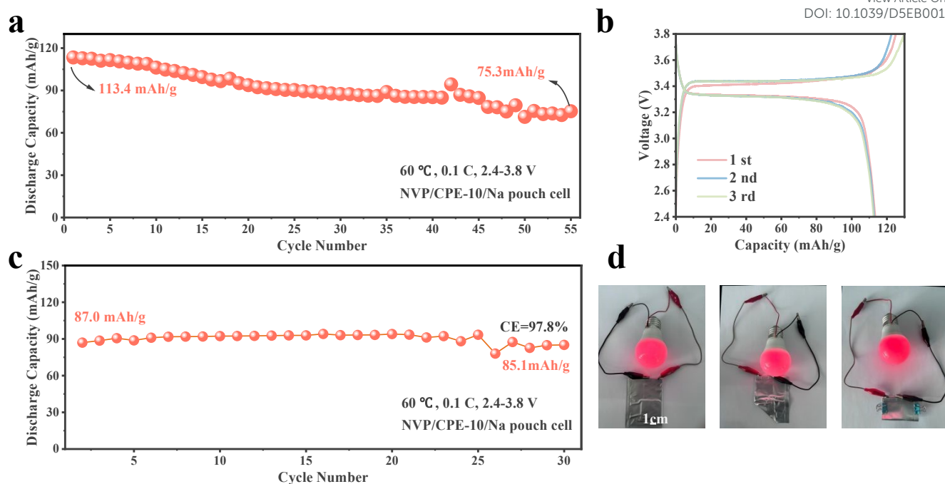
Figure 7. (a) Cycling performance of pouch-type all-solid-state NVP/CPE-10/Na cell at 0.1C with a cathode loading of 2.1 mg cm -2 . (b) Corresponding charge-discharge curves of pouch-type NVP/CPE-10/Na cell at different cycling stages. (c) Cycling performance of pouch-type all-solid-state NVP/CPE-10/Na cell at 0.1C with a cathode loading of 4.0 mg cm -2 . (d) Lighting test of the NVP/CPE-10/Na pouch cell under repeated bending and folding.
