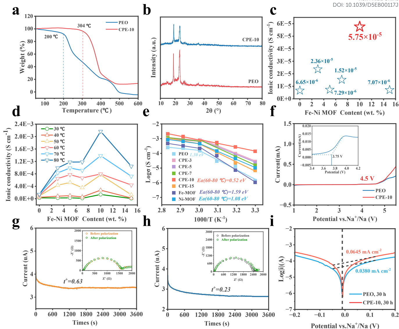
Figure 3. (a) TGA curves and (b) XRD patterns of PEO and CPE-10. (c) Ionic conductivity of CPE with different mass fractions of Fe-Ni MOF at room temperature. (d) Ionic conductivity of CPE with varying content. (e) Arrhenius plots of the ionic conductivity of CPEs. (f) LSV curves of PEO and CPE-10. (g, h) AC polarization curves of Na//Na cells using CPE-10 and PEO, with EIS (inset) before and after polarization. (i) Tafel plot comparison of Na//Na cells based on CPE-10 and PEO after 30 h of cycling.
