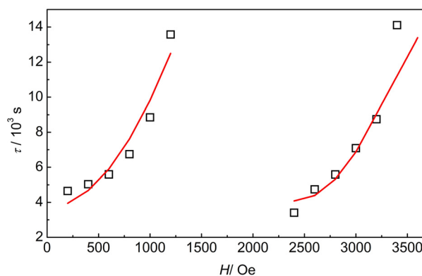
Fig. 7 \tau vs. H data plot of complex 1 arising from the 2 K AC magnetic susceptibility data. Open symbol: experimental; full line: simulated with best fitting parameters (see text).
