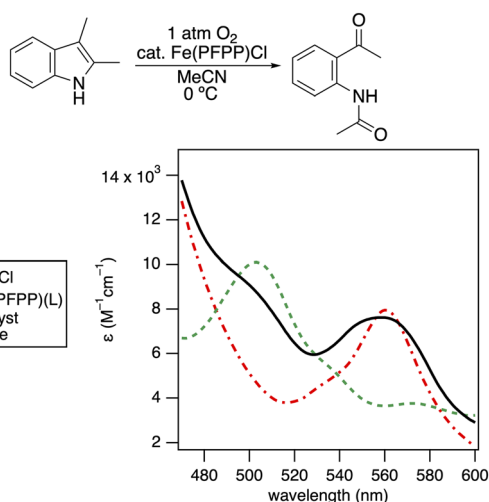
Fig. 1 UV-Vis spectrum of Q-bands of catalyst during the oxidative cleavage of 2,3-dimethyl indole (black) compared to genuine \text{Fe}(\text{PFPP})\text{Cl} (green) and \text{Fe}(\text{O}_2^-)(\text{PFPP}) (red).
