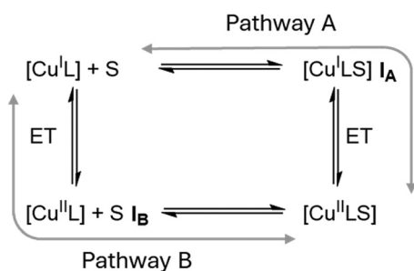
Scheme 1 Possible reaction pathways for CN-variant copper complexes as proposed by Rorabacher et al. with S denoting the external co-ligand. 37
