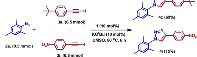
Scheme 3 Control experiments for the mechanistic investigation.
