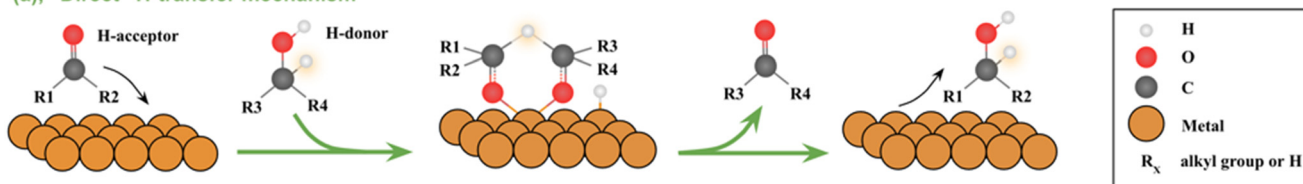
(b), “Indirect” metal hydride mechanism
