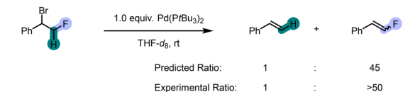
b) Determining the origin of metal-dictated chemoselectivity between \beta -hydride vs \beta -fluoride elimination
