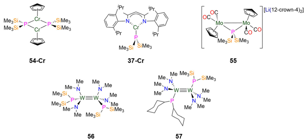
Fig. 15 Group 6 P'' complexes [Cr(Cp)(\mu-P'')]_2 ( 54-Cr ), [Cr(D^{iPr}Pacnac)(P'')] ( 37-Cr ; D^{iPr}Pacnac = CH((CH_3)_2CN(Dipp))_2 ; Dipp = C_6H_3^iPr_2-2,6 ), [Li(12-crown-4)]\{[Mo(Cp)(CO)_2]_2(\mu-P'')\} ( 55 ), [1,2-W_2(P'')(NMe_2)_4] ( 56 ), [1,2-W_2(PCy_2)(P'')(NMe_2)_4] ( 57 ).
