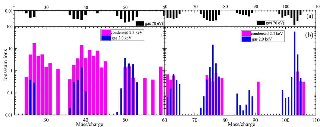
Fig. 8 Yields of cations with mass/charge from m/z = 20 – 110 produced in the gas phase and desorbed in the condensed phase (multilayer film) indicated in blue and magenta, respectively. At the top, to better highlight the differences, yields of cations formed in the gas phase by 70 eV electrons are included.
