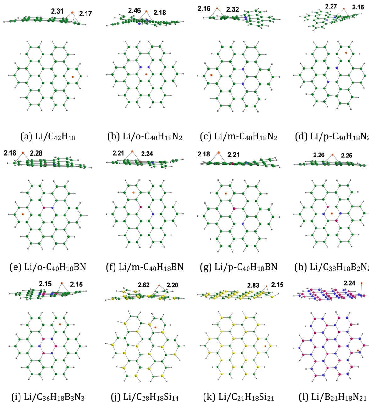
Fig. 6 Optimized structures of Li adsorbed on (a) C_{42}H_{18} , (b) o\text{-}C_{40}H_{18}N_2 , (c) m\text{-}C_{40}H_{18}N_2 , (d) p\text{-}C_{40}H_{18}N_2 , (e) o\text{-}C_{40}H_{18}BN , (f) m\text{-}C_{40}H_{18}BN , (g) p\text{-}C_{40}H_{18}BN , (h) C_{38}H_{18}B_2N_2 , (i) C_{36}H_{18}B_3N_3 , (j) C_{28}H_{18}Si_{14} , (k) C_{21}H_{18}Si_{21} , and (l) B_{21}H_{18}N_{21} . The bond distances are given in Å. The color code is the same as in Fig. 2. In addition, Li is denoted by the orange color.
