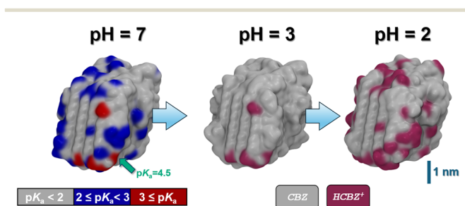
Fig. 5 Snapshots of the CBZ crystallite as obtained from MD simulations in aqueous solution (solvent not shown) at various \text{pH} values. Left: CBZ crystal at \text{pH} = 7 . A color code is used to indicate local differences in proton affinity – quantified in terms of the predicted \text{pK}_a value of the corresponding acid. While one particularly exposed CBZ experiences protonation at \text{pH} < 4.5 , we find 9 candidates for CBZ protonation at \text{pH} = 3 , as compared to 71 possible protonation sites at \text{pH} = 2 , respectively. Center & right: CBZ/CBZH core/shell nanocrystal models as obtained at \text{pH} = 3 and 2, respectively. Note that no dissociation is observed thus leading to +9 and +71 charged crystallite models of +0.005 and +0.03 \text{ C m}^{-2} surface charge density, respectively.
