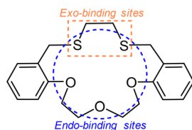
Scheme 2 Chemical structure of a ditopic O_3S_2 -macrocyclic ( L ).
