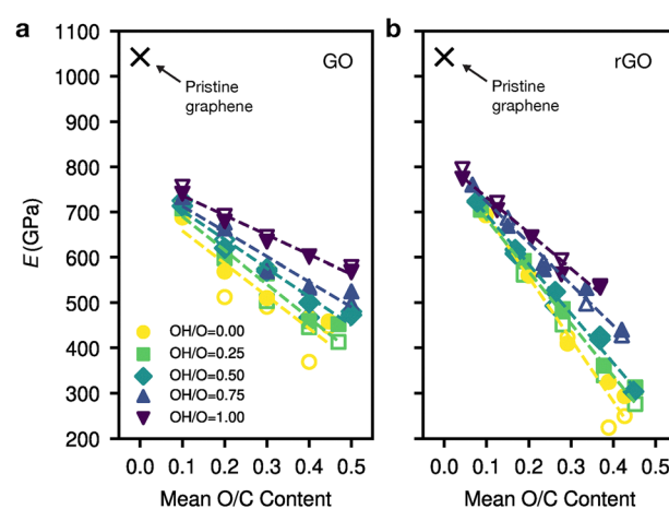
Fig. 3 Controlling the Young's modulus, E , of GO by tuning the hydroxyl content. Results are shown for varying initial OH/O ratios. (a) E values for GO: averaged for 10 structures of ~200 atoms each, strained uniaxially in x (filled markers), and 10 strained uniaxially in y (unfilled), respectively. The cross represents pristine graphene. (b) As for panel (a), except that the structures have been thermally reduced for 10 ps.
