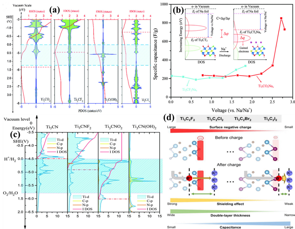
Fig. 4 (a) Relative dispositions of PDOS and integral DOS of the d-orbitals of Ti atoms in \text{Ti}_2\text{CT}_2 ( T = \text{O}, \text{F} , and \text{OH} ) and \text{Ti}_2\text{CT}_x nanosheets, (b) specific capacitance of \text{Ti}_2\text{CO}_2 and \text{Ti}_2\text{CF}_2 nanosheets, 49 (c) relative PDOS and integral DOS of the d-orbitals of Ti atoms referenced to the standard hydrogen electrode (SHE), 50 and (d) schematic showing the electronic impact of the MXene electrode surface on EDL capacitances depending on the surface functional groups. 51
