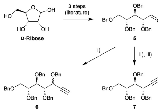
Scheme 1 Synthesis of alkyne-tagged probe scaffolds. (i) Ethylmagnesium bromide, TMS-acetylene, THF, -78 °C to rt; then NaH, BnBr, THF, 0 °C to rt, 58% over two steps (dr 3.5:1). (ii) \text{CBr}_4 , \text{PPh}_3 , \text{Et}_3\text{N} , \text{CH}_2\text{Cl}_2 , -10 °C to rt, 84%. (iii) LDA, THF, 72%.
