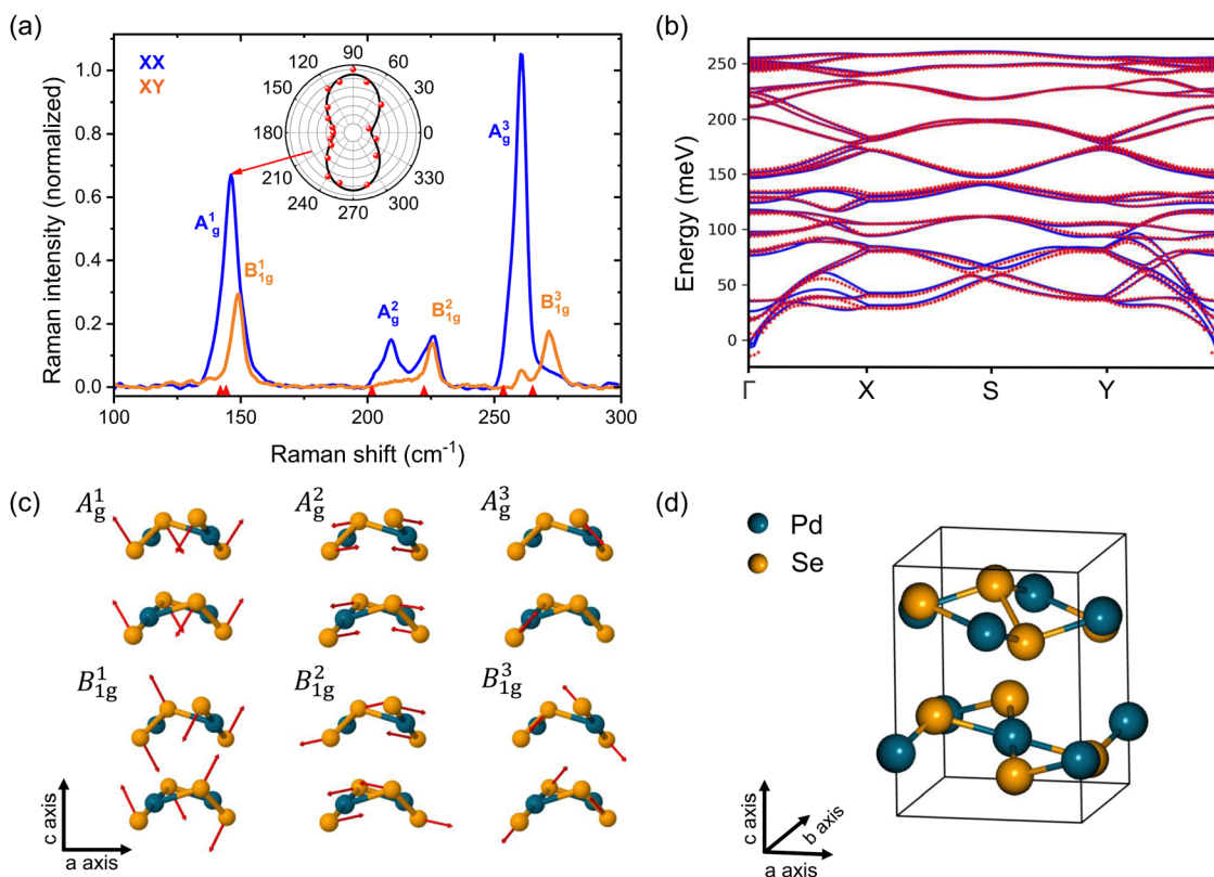
Fig. 1 (a) Raman spectra of bulk PdSe 2 in parallel (blue line) and cross configurations (yellow line) at room temperature. Phonon modes are labeled with an irreducible representation. The inset shows the polarization-dependence of the Raman intensity of A g 1 under parallel configurations (scattered dots). The fit of the Raman intensities versus polarization angles (black line). The vertical red arrows indicate the phonon frequencies calculated by DFT. (b) DFPT calculation of the phonon dispersion of bulk PdSe 2 (blue) compared to the dispersion calculated via the EPW code used to obtain the electron–phonon coupling (red). (c) Atomic displacements corresponding to the phonon modes of PdSe 2 , as depicted, projected along the b -axis and showing two layers, to indicate the phase relationship between layers. (d) The crystal structure of PdSe 2 unit cell.
