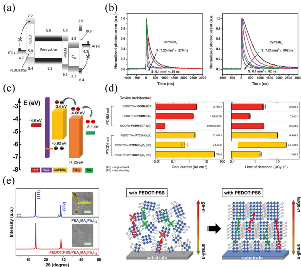
Fig. 10 (a) Energy diagram of the cross-linked OTPD MHPDs. Reproduced with permission. 10 Copyright 2015, Wiley-VCH. (b) Transient response curves of the inorganic MHPDs with PTA/PEIE. Reproduced with permission. 106 Copyright 2018, Wiley-VCH. (c) Energy band diagram of the MHPDs with ultrathin Al 2 O 3 and TiO 2 modification layers. Reproduced with permission. 107 Copyright 2019, Wiley-VCH. (d) Summary of the interface engineering based on several organic materials. Reproduced with permission. 108 Copyright 2020, Wiley-VCH. (e) XRD patterns of quasi-2D thin films without and with PEDOT:PSS interlayer (left), the insets are the corresponding top-view FESEM images (scale bar: 1 μm), and schematic illustration of the orientational growth of MHP films without/with PEDOT:PSS interlayer. Reproduced with permission. 109 Copyright 2023, Wiley-VCH.
