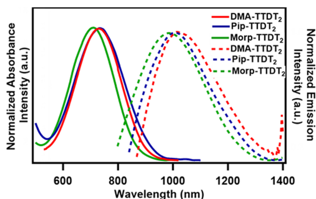
Fig. 2 Normalized absorbance (solid lines) and emission (dashed lines) spectra of the TTDT 2 based fluorophores in 10^{-5} M \text{CHCl}_3 .
