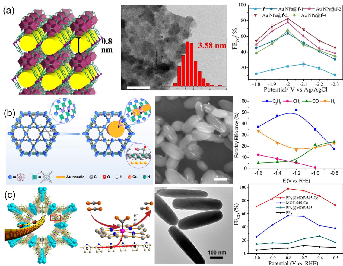
Fig. 7 (a) Three-dimensional framework of 1' , TEM image of Au-NPs@ 1' - 3 and FE_{CO} of Au NPs@ 1' - x ( x = 1, 2, 3 , and 4 ). 51 Copyright 2022, Wiley-VCH. (b) Schematic illustration, the SEM image and FE for different products of the AuNN@PCN-222(Cu) catalyst. 188 Copyright 2022, Springer Nature. (c) Schematic illustration for the advantages of PPy in MOF-545-Co, the TEM image of PPy@MOF-545-Co and FE_{CO} of PPy@MOF-545-Co at different voltages. 189 Copyright 2021, American Chemical Society.
