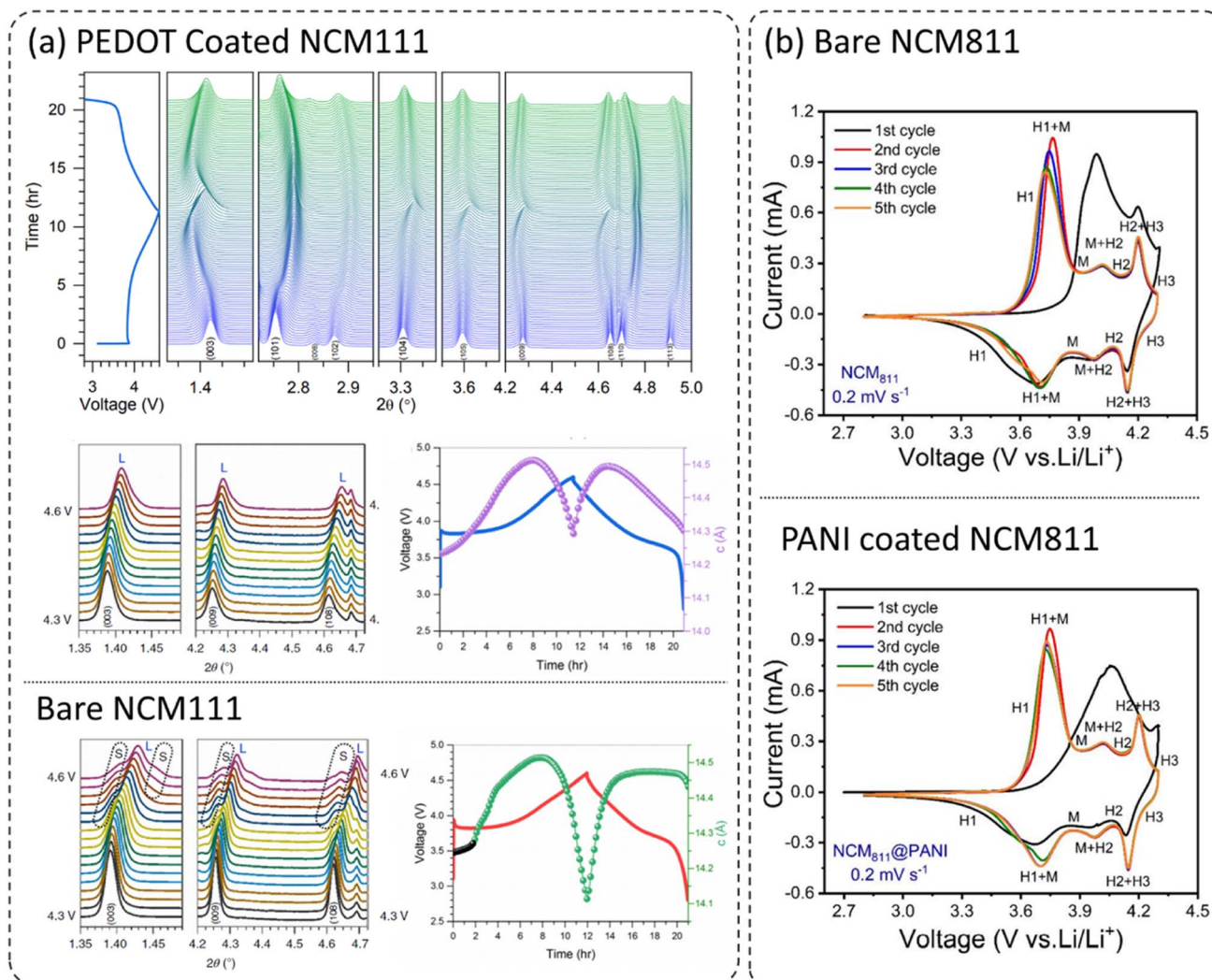
Fig. 4 (a) In situ HEXRD patterns of the PEDOT coated \text{NCM}_{111} cathode during the 1st charge/discharge cycle within 2.8–4.6 V. Later, the HEXRD patterns of bare and PEDOT coated \text{NCM}_{111} in the voltage region of 4.3–4.6 V during the charge at C/10 , and the change in the lattice parameter 'c' as a function of charge/discharge time. L and S correspond to the layered and spinel phases, respectively, 26 reproduced from ref. 26 with permission from Nature Portfolio, copyright 2019, (b) CV curves for the five cycles at 0.2 \text{ mV s}^{-1} (2.8–4.3 V) for bare and PANI coated \text{NCM}_{811} , 23 reproduced from ref. 23 with permission from American Chemical Society, copyright 2019.
