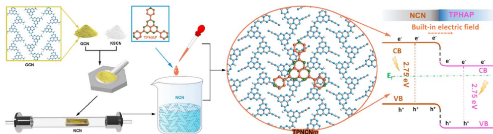
Scheme 1 Schemed fabrication process of the TPNCN m photocatalyst.
