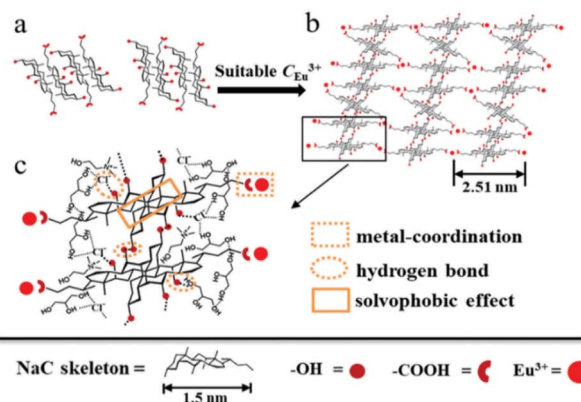
Fig. 27 Sketch of the self-assembly route and intermolecular interactions in the \text{Eu}^{3+} /NaC/ChCl–Gly eutectogel. (a) Scheme of NaC dimers; (b and c) self-assembly of NaC/ChCl–Gly in the presence of \text{Eu}^{3+} and details of the type of interactions. Reproduced from M. Sun, Q. Li and X. Chen, Self-assembled luminescent cholate gels induced by a europium ion in deep eutectic solvents, Soft Matter , 2021, 17, 2815–2822, with permission from the Royal Society of Chemistry.
