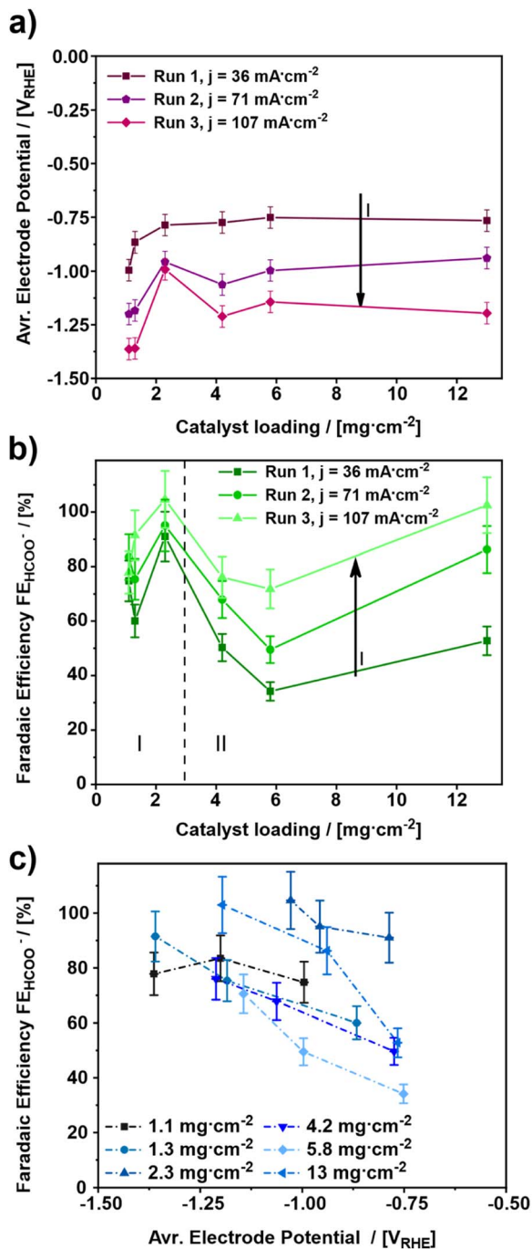
Fig. 1 Influence of the catalyst loading on (a) the average electrode potential for three different applied current densities (36, 71 and 107 \text{mA}\cdot\text{cm}^{-2} ) and (b) the faradaic efficiency for formate after a run time of 11 min each. (c) Shows a combination of the plots a and b. (Measurement conditions: batch reactor, 12 ml electrolyte, 1 M \text{KHCO}_3 , continuous \text{CO}_2 supply of 20 \text{ml}\cdot\text{min}^{-1} , start at room temperature, electrolysis time: 45 min each).
