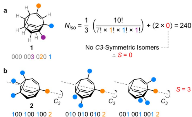
Fig. 2 Structural formulae and isomer barcodes of (a) one of the 240 unique isomers of BV 1, showing the calculation of N_{\text{iso}} , and (b) the three C_3 -symmetric isomers of BV 2 that are accounted for by a correction factor of S = 3 .
