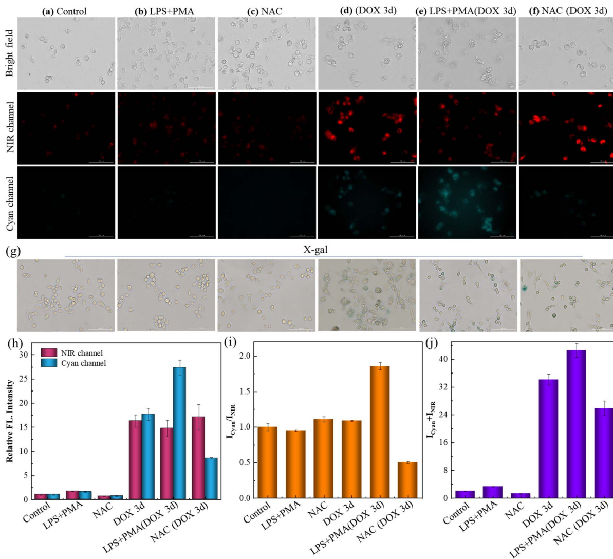
Fig. 3 (a–f) Fluorescent images of RAW 264.7 cells after incubation with 10 \mu M SA-HCy-1. (a) The control group (normal RAW 264.7 cells); (b) the cells were pretreated with LPS ( 1.0 \mu\text{g mL}^{-1} ) and PMA ( 0.5 \mu\text{g mL}^{-1} ) for 60 min; (c) the cells were pretreated with NAC (10 mM) for 60 min; (d) the cells were pretreated with DOX ( 0.1 \mu\text{M} ) for 3 days; (e) the cells were pretreated with 0.1 \mu\text{M} DOX for 3 days and then treated with LPS ( 1.0 \mu\text{g mL}^{-1} ) and PMA ( 0.5 \mu\text{g mL}^{-1} ) for 60 min. (f) The cells were pretreated with 0.1 \mu\text{M} DOX for 3 days and then treated with NAC (10 mM) for 60 min. Top: bright field; middle: NIR channel; ground: cyan channel. For the NIR channel: \lambda_{\text{ex}} = 628 \text{ nm} , \lambda_{\text{em}} = 670\text{--}730 \text{ nm} ; for the cyan channel: \lambda_{\text{ex}} = 377 \text{ nm} , \lambda_{\text{em}} = 450\text{--}500 \text{ nm} , scale bar = 100 \mu\text{m} . (g) X-gal staining of RAW 264.7 cells with different treatments of (a–f). (h) Relative fluorescence intensities of (a)–(f) from NIR (red bars) and cyan (blue bars) channels. (i) Quantification of fluorescence intensity ratios ( I_{\text{Cyan}}/I_{\text{NIR}} ) of the images from (a)–(f). (j) Quantification of fluorescence intensity sums ( I_{\text{Cyan}} + I_{\text{NIR}} ) of the images from (a) to (f). Error bars represent the standard deviation ( \pm S.D.), n = 3 .
