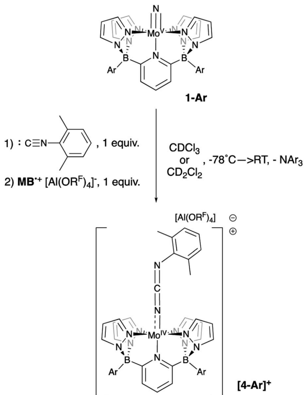
Scheme 6 Reaction of 1-Ar with 1 equivalent of oxidant at -78^\circ\text{C} in the presence of xyllyl isocyanide.
