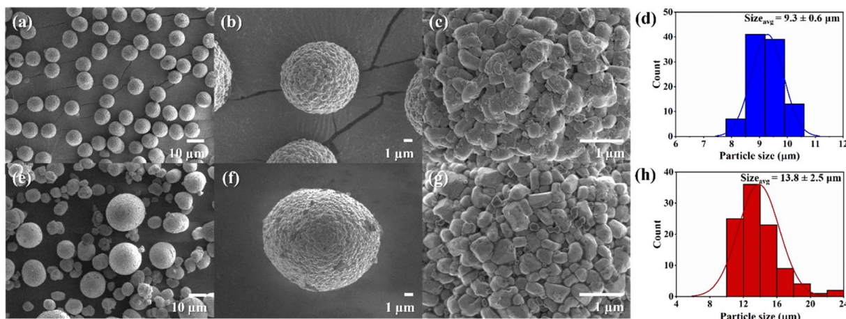
Fig. 1 Top-view FESEM images with different magnifications of the (a)–(c) NMC90 powder and (e)–(g) the NMC80 powder and the particle size distribution of the (d) NMC90 and (h) NMC80 powders.
