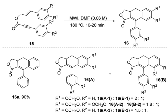
Scheme 3 Synthesis of ADHNs through DMF-regulated intramolecular dehydro-Diels–Alder reactions of styrene-yne.
