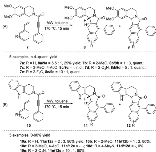
Scheme 1 Synthesis of ADHNs via microwave-assisted intramolecular Diels–Alder reactions of styrene-yne.
