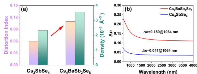
Fig. 6 (a) Comparison of the tetrahedral distortion index and functional unit density between CSS and CBSS; and (b) the calculated birefringence of CSS and CBSS.
