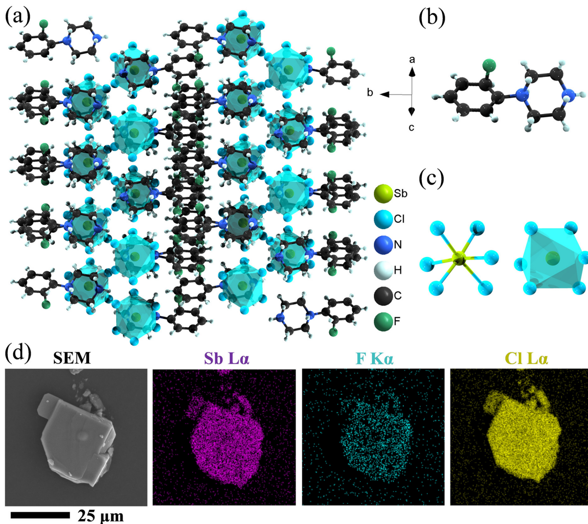
Fig. 1 The structural characterization of [FPPP] 2 SbCl 7 . (a) The arrangement of molecules in the prepared 0D sample as viewed towards the [101] plane. Structural diagrams of the [FPPP] 2+ cation (b) and the [SbCl 6 ] 3- octahedron (c). (d) SEM images and the corresponding mapping of elements of the prepared microparticles, respectively.
