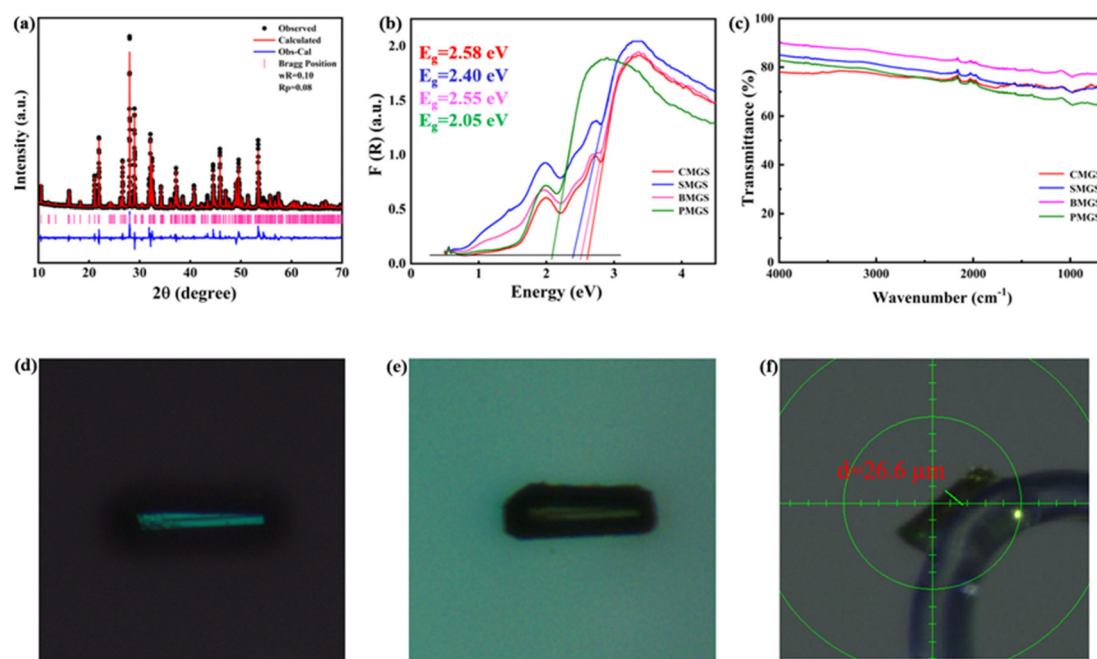
Fig. 3 (a) Rietveld refinement of the powder XRD profile for CMGS; (b) band gaps of \text{MMn}_6\text{Ga}_6\text{S}_{16} ( M = \text{Ca}, \text{Sr}, \text{Ba}, \text{Pb} ); (c) IR spectra of \text{MMn}_6\text{Ga}_6\text{S}_{16} ( M = \text{Ca}, \text{Sr}, \text{Ba}, \text{Pb} ); and (d–f) the original interference color, extinction, and thickness of the CMGS crystal, respectively.
