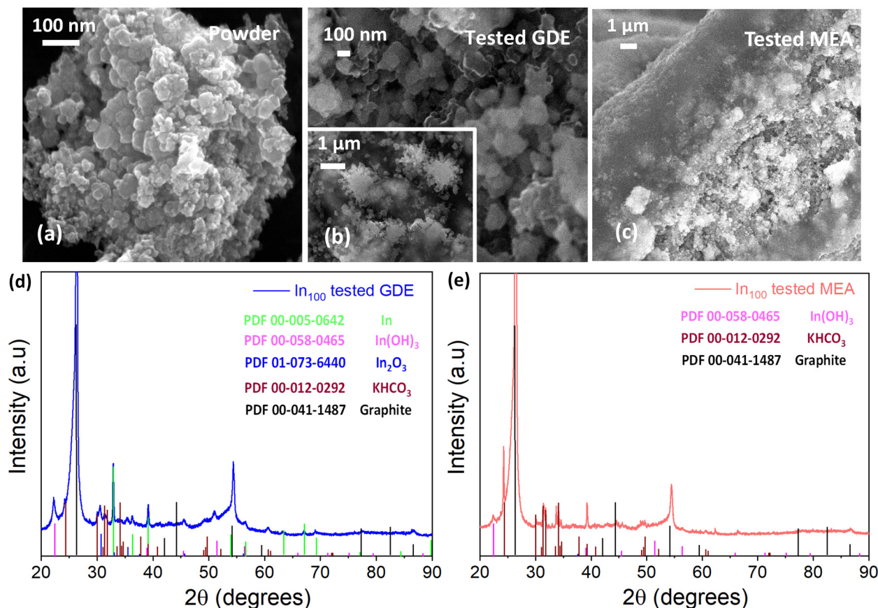
Fig. 15 In 100 catalyst: SEM images of (a) fresh nanopowder; (b) after electrochemical CO 2 reduction in the GDE system; (c) after electrochemical CO 2 reduction in the MEA system; (d) XRD pattern obtained on the post-mortem GDE electrode, and (e) XRD pattern obtained at Eni SpA in the post-mortem MEA electrode.
