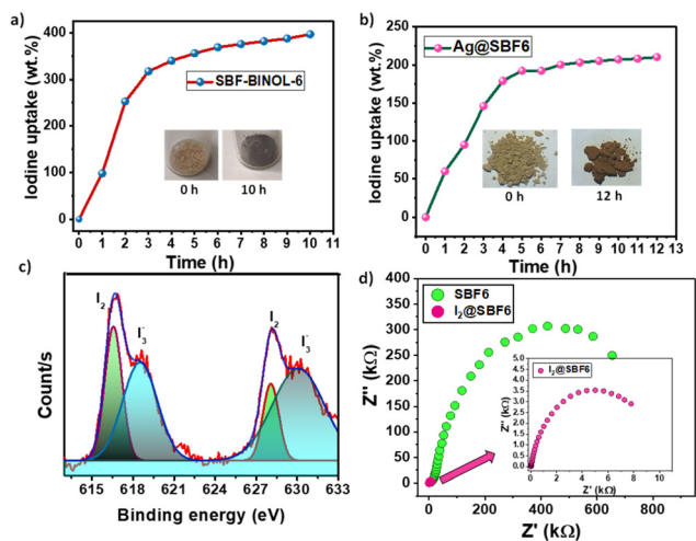
Fig. 4 Iodine vapor uptake with time for (a) SBF-BINOL-6 ; (b) Ag@SBF6 . (c) Deconvoluted XPS spectra for iodine in \text{I}_2\text{@SBF6} . (d) The Nyquist plot for SBF-BINOL-6 and \text{I}_2\text{@SBF6} (inset).
