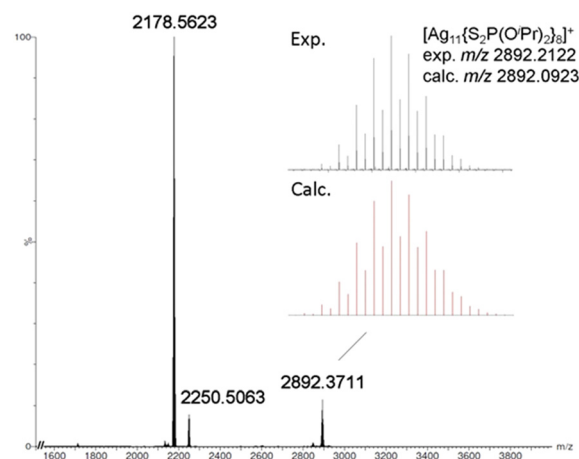
Fig. 1 The positive-ion ESI-MS of Ag 11 .
