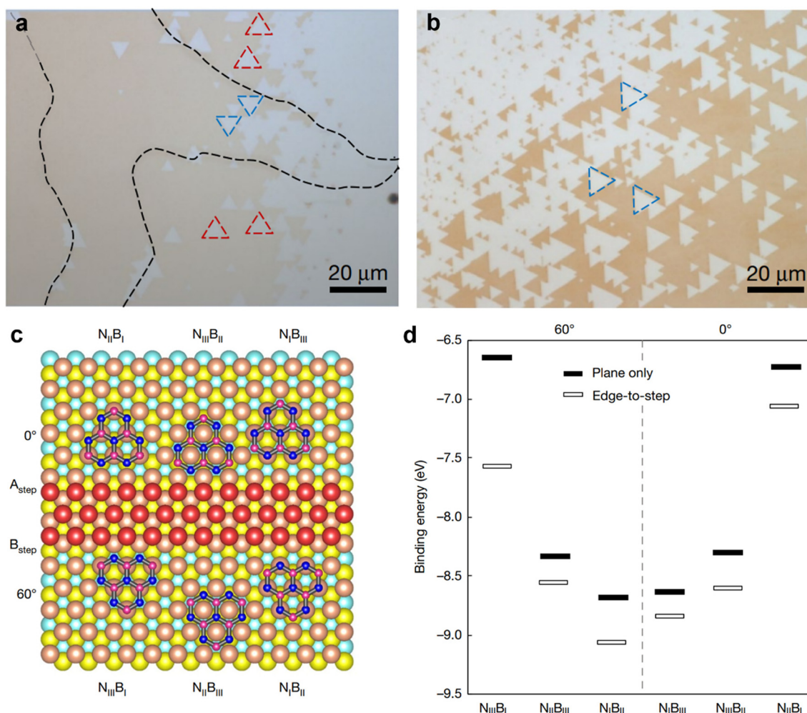
Fig. 5 (a) OM image of monolayer hBN triangular flakes grown on a Cu (111) thin film with 60^\circ in-plane rotated twin grains marked by blue and red dotted triangles. (b) OM image of unidirectionally aligned monolayer hBN triangular flakes grown on a Cu (111) thin film. (c) The lowest-energy atomic arrangements of six B_6N_7 -Cu (111) units, considering the edge docking to two opposite step-edge terminations (A and B) of top-layer Cu (111). (d) Calculated binding energies for the six B_6N_7 -Cu (111) configurations, with and without including the edge-to-step epitaxy effect. [Fig. (a–d) are reproduced with permission from Chen et al. 22 Copyright 2020, rights managed by the Nature Publishing Group].
