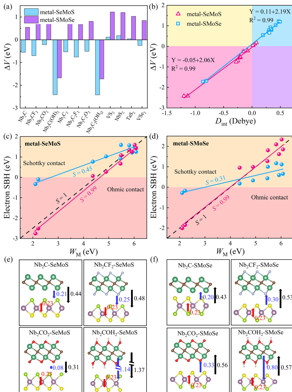
Fig. 4 (a) The electronic potential difference ( \Delta V ) in 2D metal-MoSSe contacts. (b) The change in \Delta V with interface dipole ( D_{\text{int}} ) for 2D metal-MoSSe contacts. The variation in the electron SBH as a function of metal work functions ( W_M ) for (c) metal-SeMoS (d) metal-SMoSe contacts. The azure and pink lines represent fitting results without and with \Delta V correction, respectively. The black dotted line represents the Schottky-Mott limit S = 1 . The Fermi level pinning factor S is defined as the value of the fitted slope. The dipole moment distributions in selected (e) 2D metal-SeMoS and (f) 2D metal-SMoSe contacts. The red, blue, and black arrows represent the intrinsic dipole, interface dipole, and total dipole, respectively.
