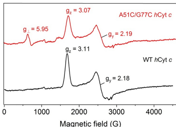
Fig. 7 EPR spectra of ferric WT (black) and A51C/G77C (red) hCyt c (0.3 mM), collected at 20 K, 2 mW power and 9.4 GHz.
